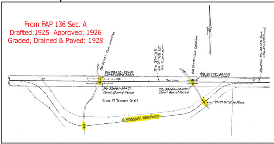
Example of how the early, unimproved roadway often went around terrain obstacles.
